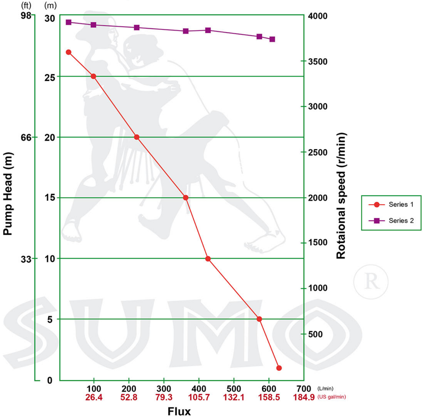
Pump Performance curve
